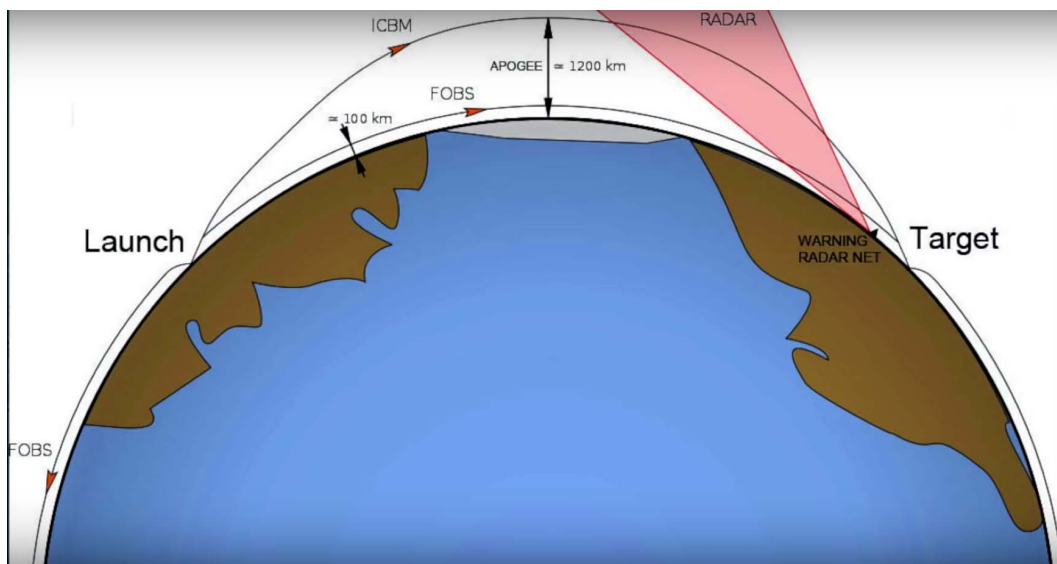
Figure 87. A North Pole low orbit (100 km) Fractional Orbital Bombardment System (FOBS) ICBM or cruise missile trajectory reduces the radar warning time compared with a high ICBM orbit (1,200 km) trajectory.
