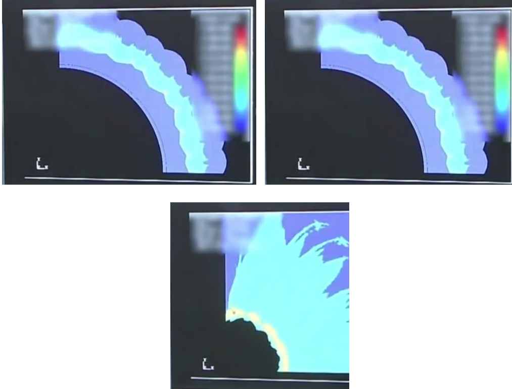
Figure 31. Multipoint hemisphere initiation U^{235} hydrodynamic implosion simulations.
