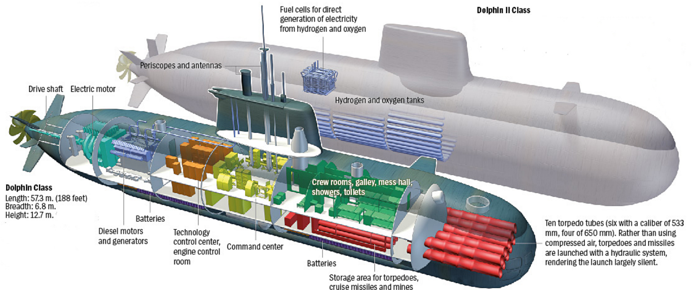
Figure 37. The Dolphin II class of submarines is equipped with modern diesel-electric propulsion and uses silent fuel cells using hydrogen and oxygen for electrical propulsion allowing it to remain submerged for several weeks. The Dolphin I and II use silent hydraulic instead of compressed air torpedo and cruise missile launching systems. Decks 2 and 3 are where the nuclear devices would be stored. Source: DPA.
