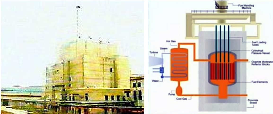
Figure 7. Exterior view of the Yongbyon 1, 5 MWth gas cooled graphite research reactor in the DPRK.
