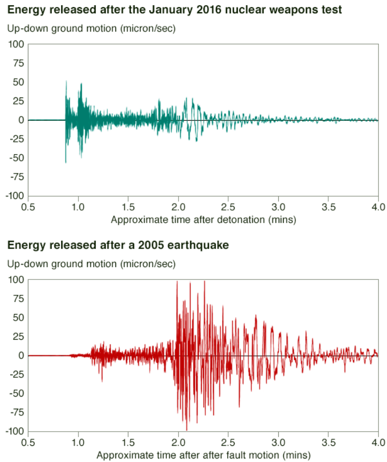
Figure 10. Distinction between underground nuclear tests and earthquakes signatures. Two peaks are associated with nuclear devices the first being the nuclear explosive followed by the collapse of the created molten rock cavity. Source: Incorporated Research Institute for Seismology, BBC.
