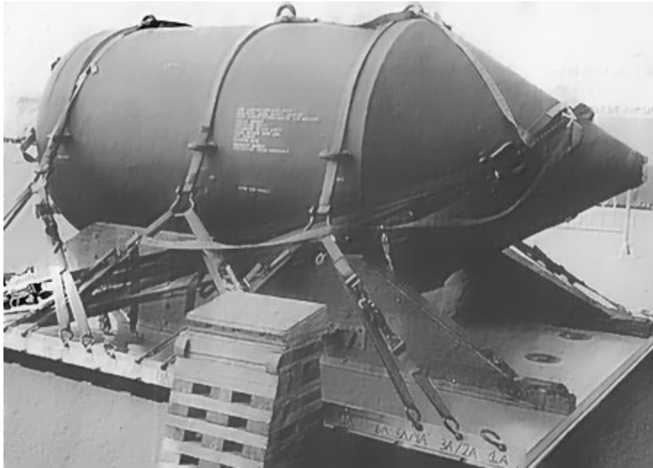
Figure 51. A 15,000 pounds Daisy-Cutter BLU-82 device on its parachute-dropping pallet.
