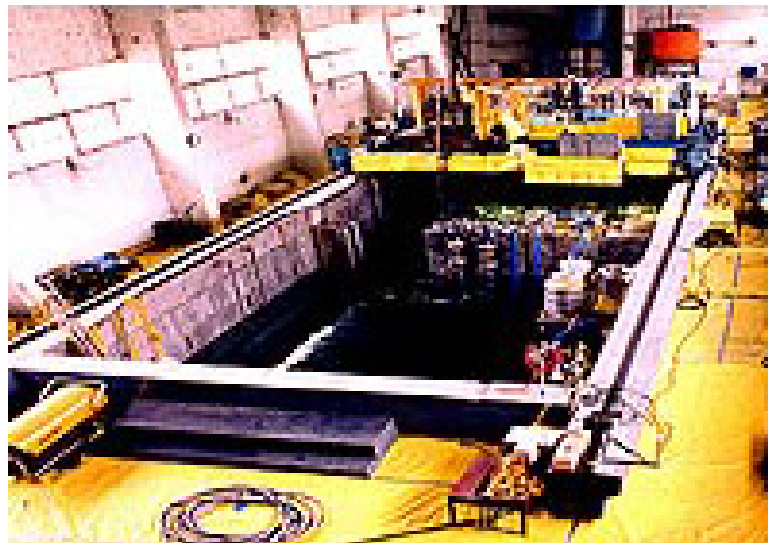
Figure 6. Fuel storage pool of Yongbyon-1, 5 MWth research reactor in the DPRK. AP Photograph.
