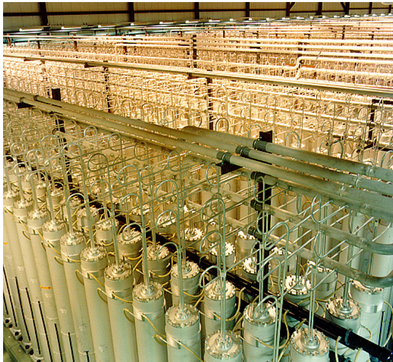
Figure 24. Urenco U 235 enrichment gas centrifuges cascade.
