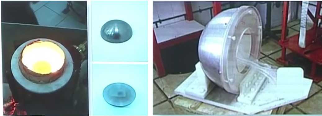
Figure 30. Multipoint initiation implosion experiments on a uranium hemisphere were discontinued in 2003. U^{235} is imploded rather than Pu^{239} , possibly based on Pakistani or North Korean configurations.
