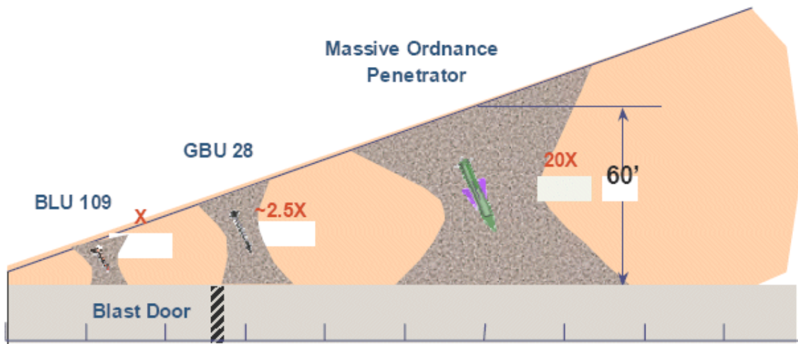
Figure 71. Concrete penetration of 20,000-30,000 lbs of blast, penetrator and parafoil deployed vehicle variants of earth penetrator munitions.
