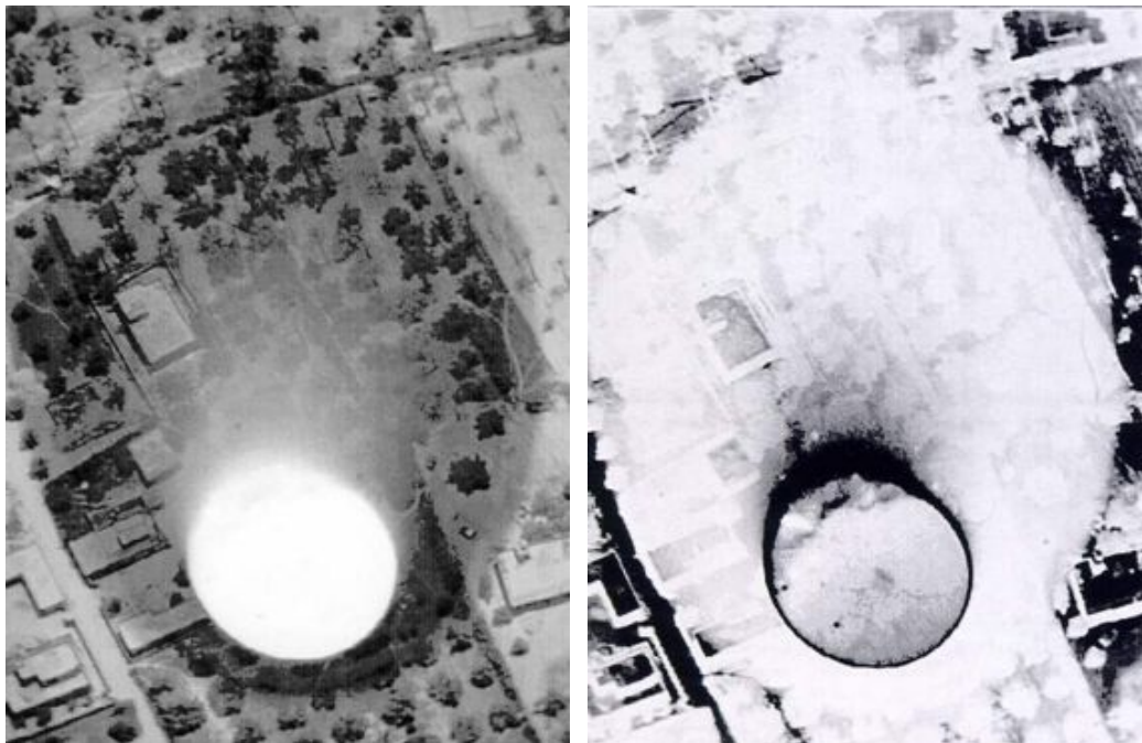
Figure 77. Far-end of the visible spectrum approaching the ultraviolet spectrum a few hundreds of a microsecond (left) at its brightest, and one millisecond later (right) into the detonation of a low-yield 1 kT of TNT equivalent Enhanced Radiation Device (ENRD, neutron bomb) device
