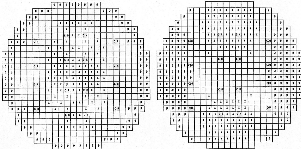
Figure 11. Initial radial power distribution (left) and radial power distribution at the time of the power excursion (right). CR: control rods, x: P > 1.3 P_{\text{average}} , \phi : P < 0.7 P_{\text{average}} . At the time of the accident, the core had split into two cores.
