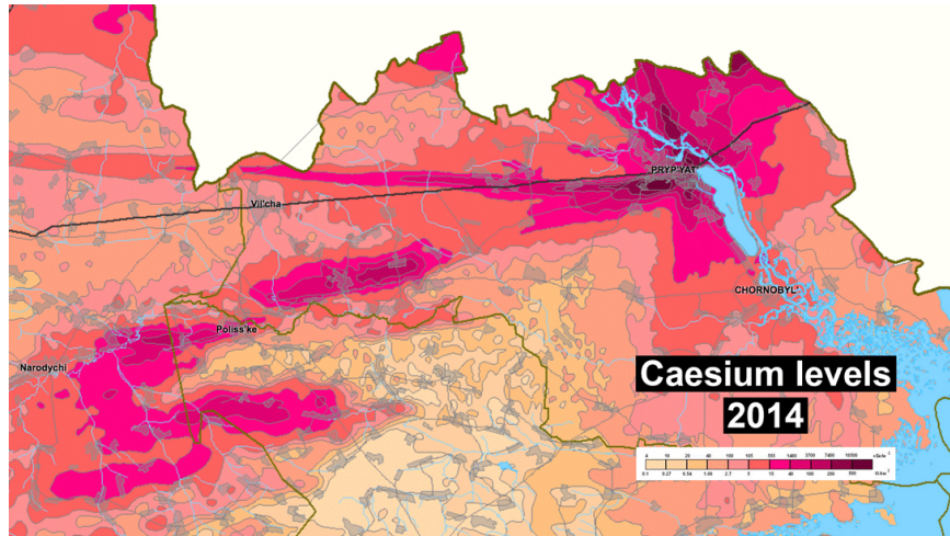
Figure 19. Reduction of the Cs^{137} soil levels around Chernobyl, 1986 to 2014.
