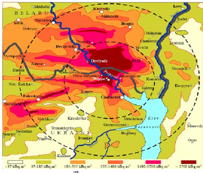
Figure 18. Initial \text{Cs}^{137} deposition round the town of Prip'yat and Chernobyl.
