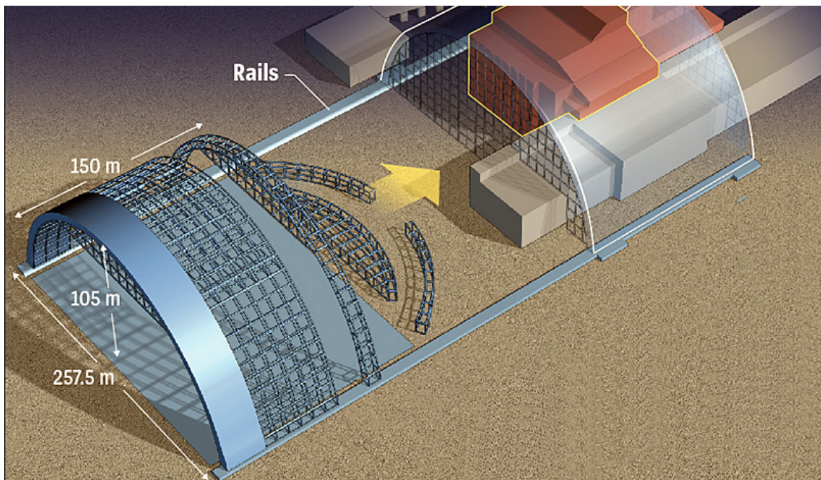
Figure 20. Metallic vault for the damaged Chernobyl unit 4 reactor. The metallic shield was constructed near the reactor then moved on rails to cover it. Source: Der Spiegel.
