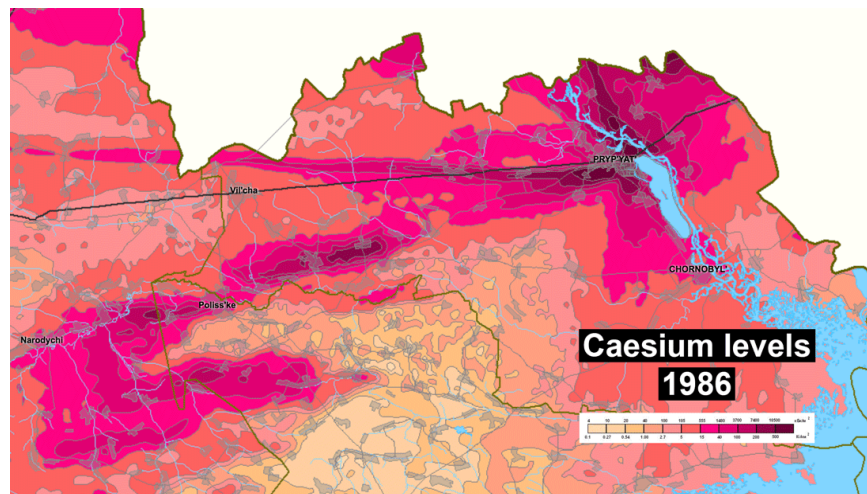
Figure 18. Initial \text{Cs}^{137} deposition round the town of Prip'yat and Chernobyl.
