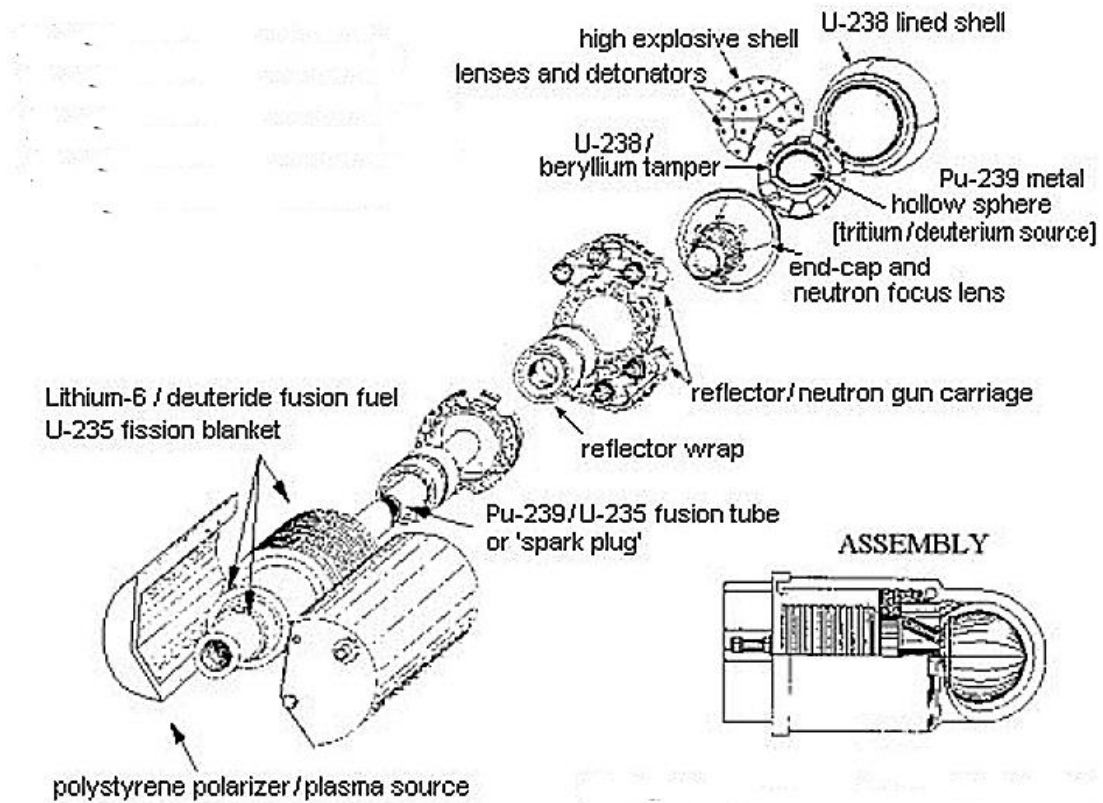
Figure 57. UK assumed design of a staged thermonuclear device. Source: Greenpeace.
