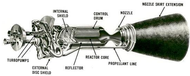
Figure 11. NERVA solid core rocket design.
