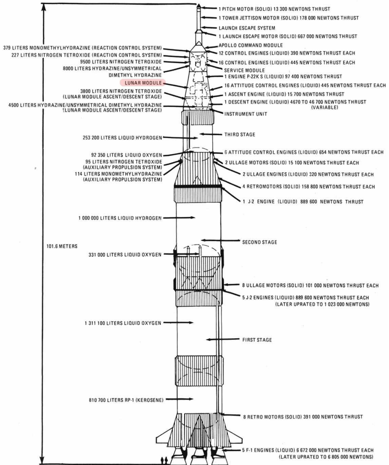
Figure 21. Saturn V rocket used in Apollo Program missions to the moon. Source: NASA.
