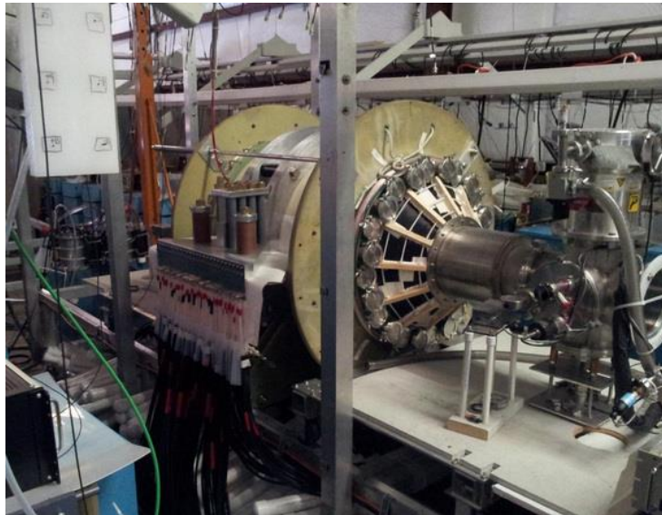
Figure 18. Fusion rocket experiment. Source: Univ. of Washington.
