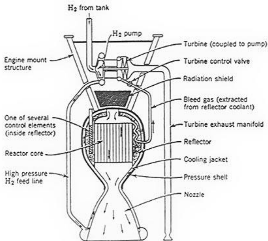
Figure 10. Solid Reactor Core for Nuclear Thermal Propulsion, NPT.
