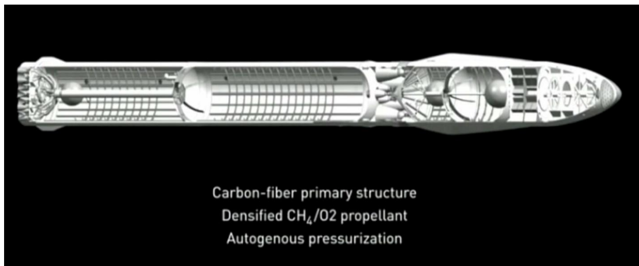
Figure 40. Mars ship cross section. Source: Space X.
