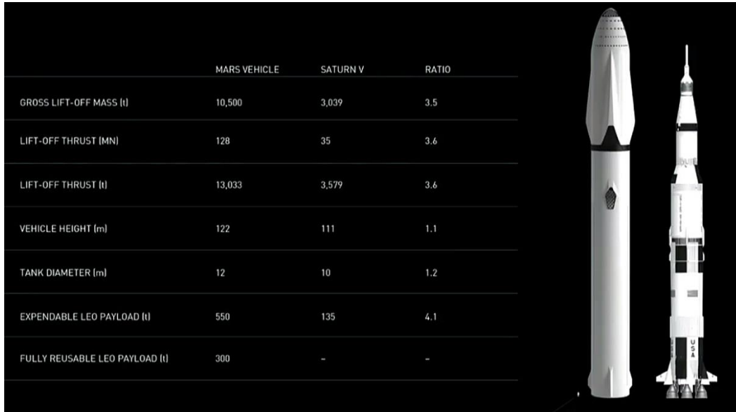
Figure 39. Comparison of NASA Saturn V Apollo missions to the moon rocket and Space X Mars Interplanetary Transport System (ITS). Source: Space X.
