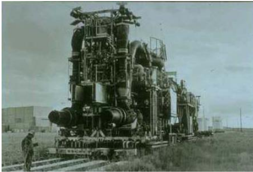
Figure 25. Nuclear Jet airplane engine at Idaho National Engineering Laboratory (INEL).
