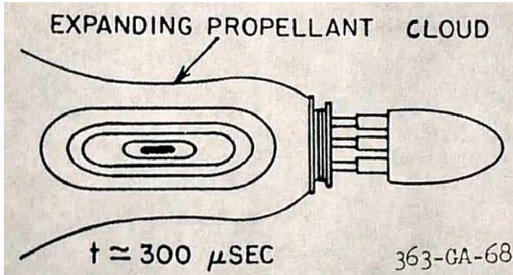
Figure 37. Expanding propellant cloud in the Orion concept. Source: General atomics.
