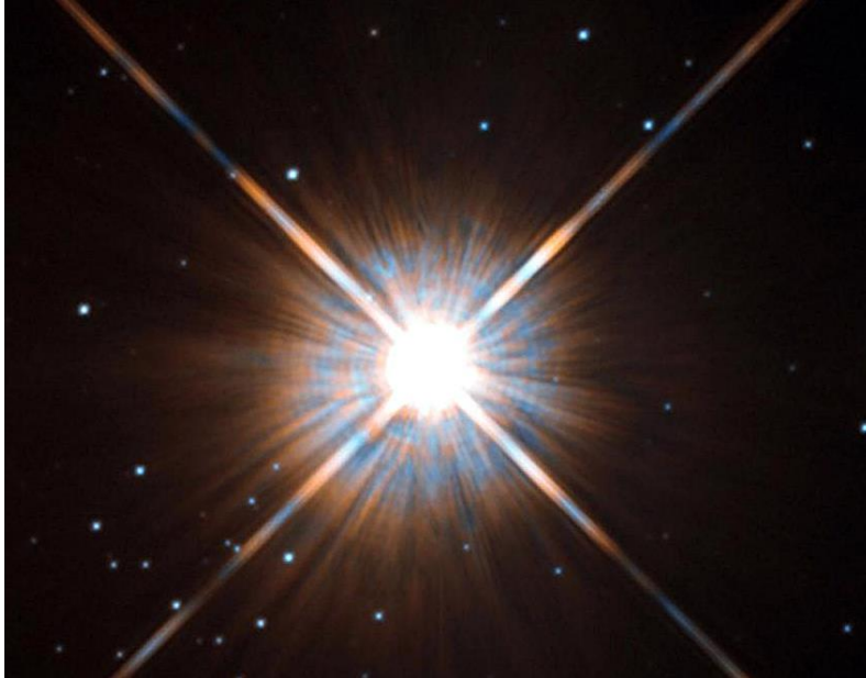
Figure 50. Proxima Centauri. Source: ESA/Hubble.
