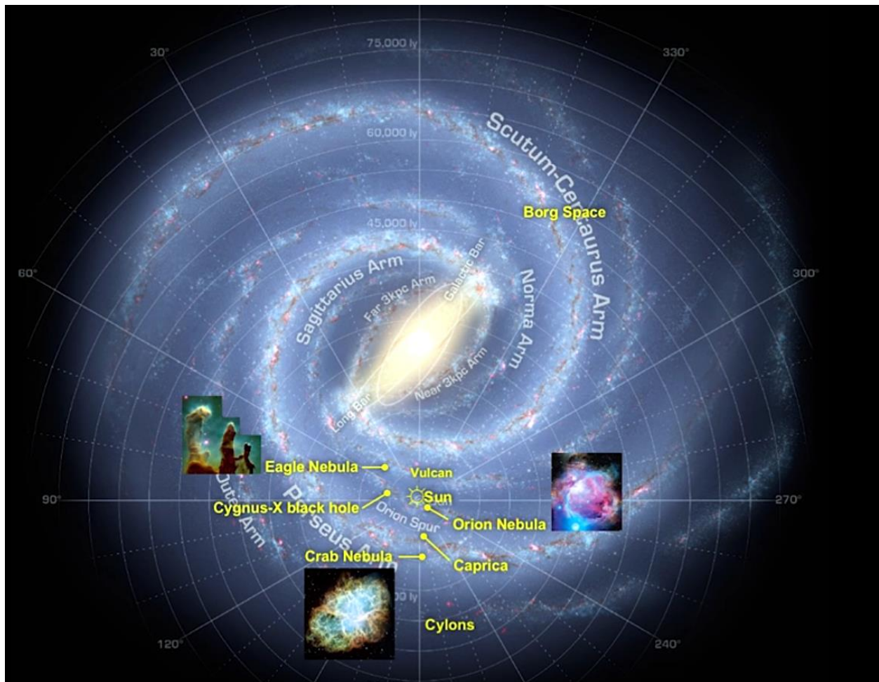
Figure 6. Milky Way galaxy.
