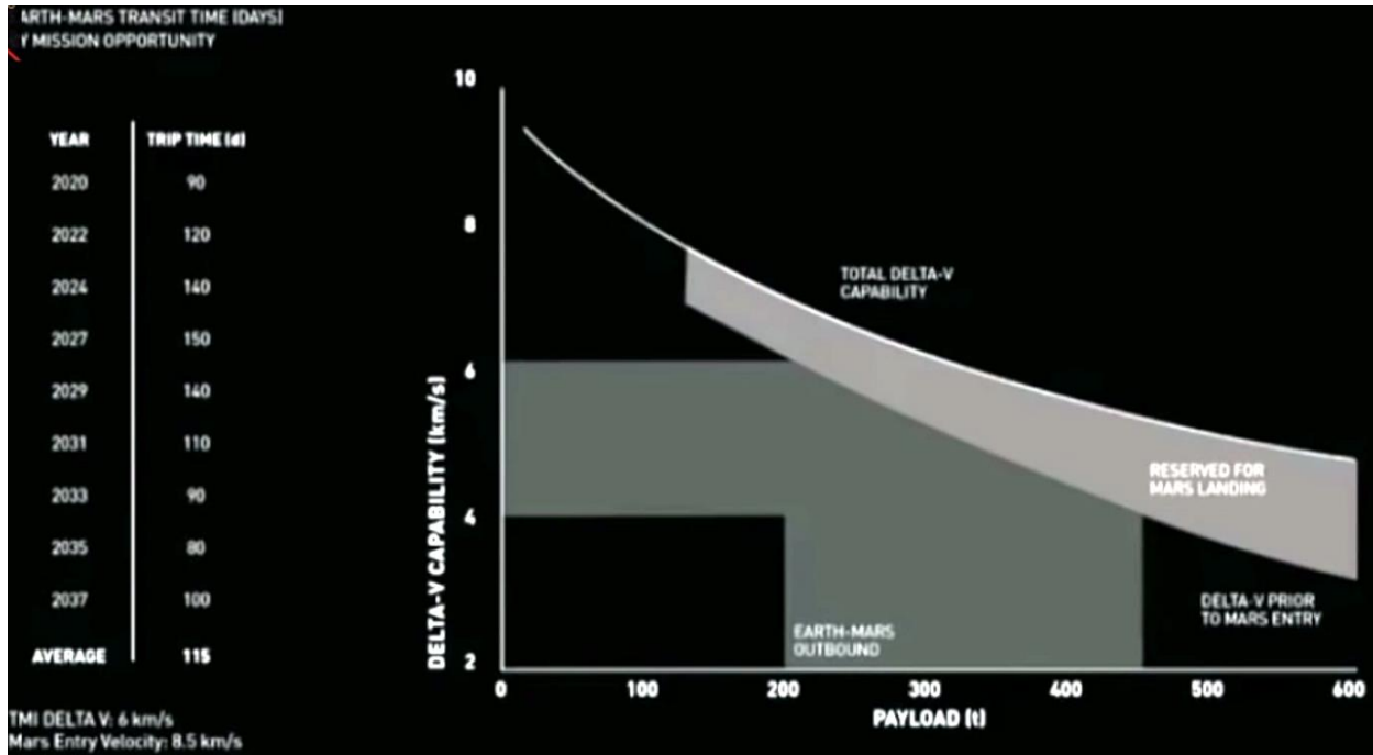
Figure 46. Transit time for a Mars mission. Source: Space X.
