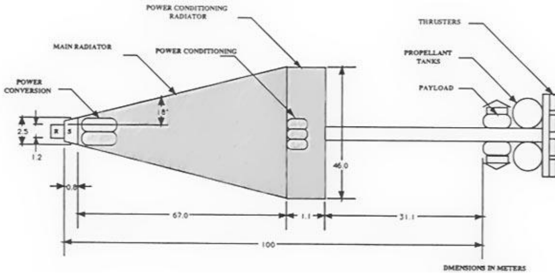
Figure 14. Schematic of Nuclear Electric Propulsion, NEP Vehicle and System.
