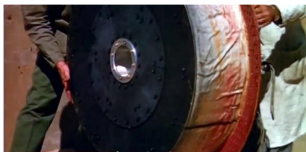
Figure 32. Orion pusher plate design. Source: GA.
