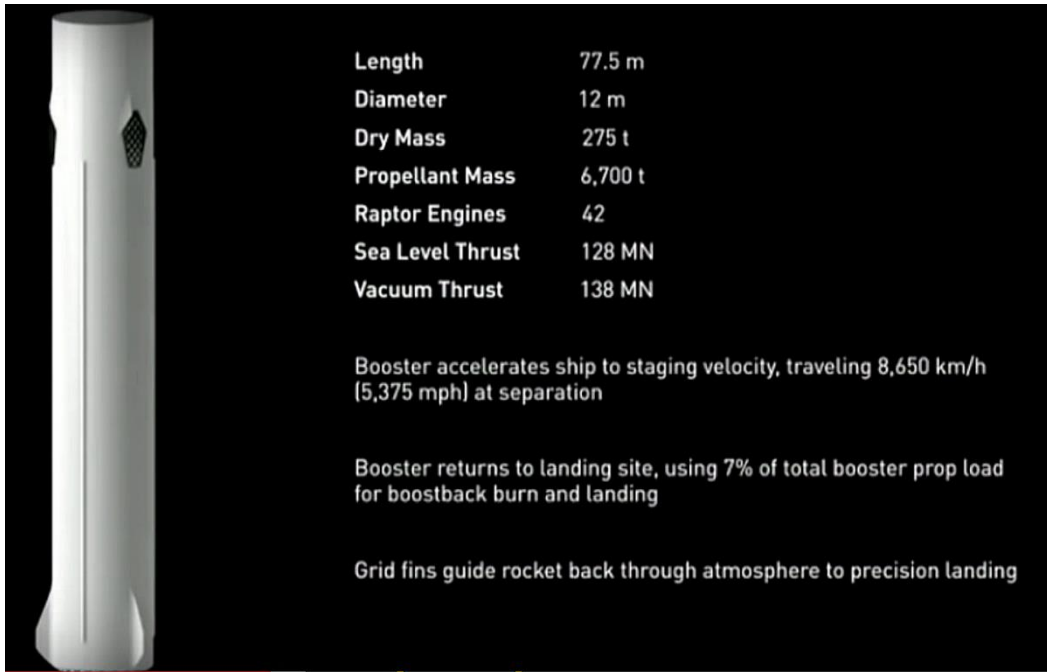
Figure 42. Reusable booster specifications. Source: Space X.
