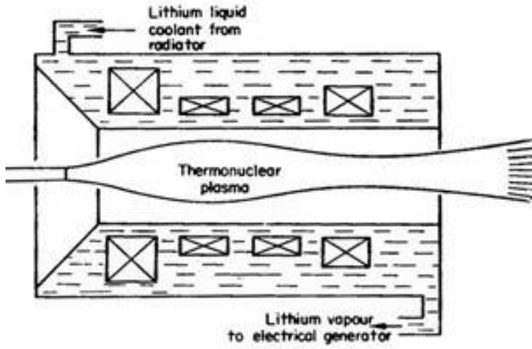
Figure 17. Schematic of a nuclear fusion rocket.
