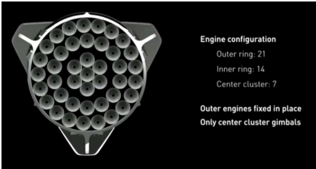
Figure 44. Raptor engines cluster. Source: Space X.
