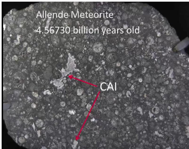
Figure 51. Allende meteorite.
