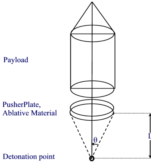
Figure 35. Geometry for the External Pulsed Plasma Propulsion, EPPP Rocket.
