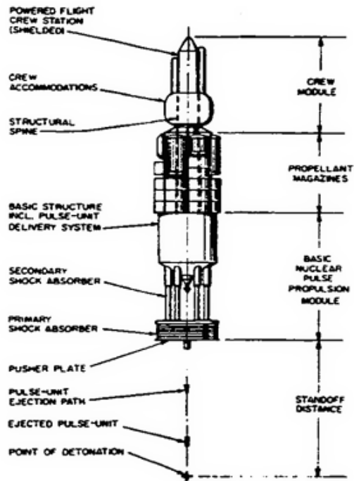
Figure 31. An External Pulsed Plasma Propulsion, EPPP Space Vehicle.
