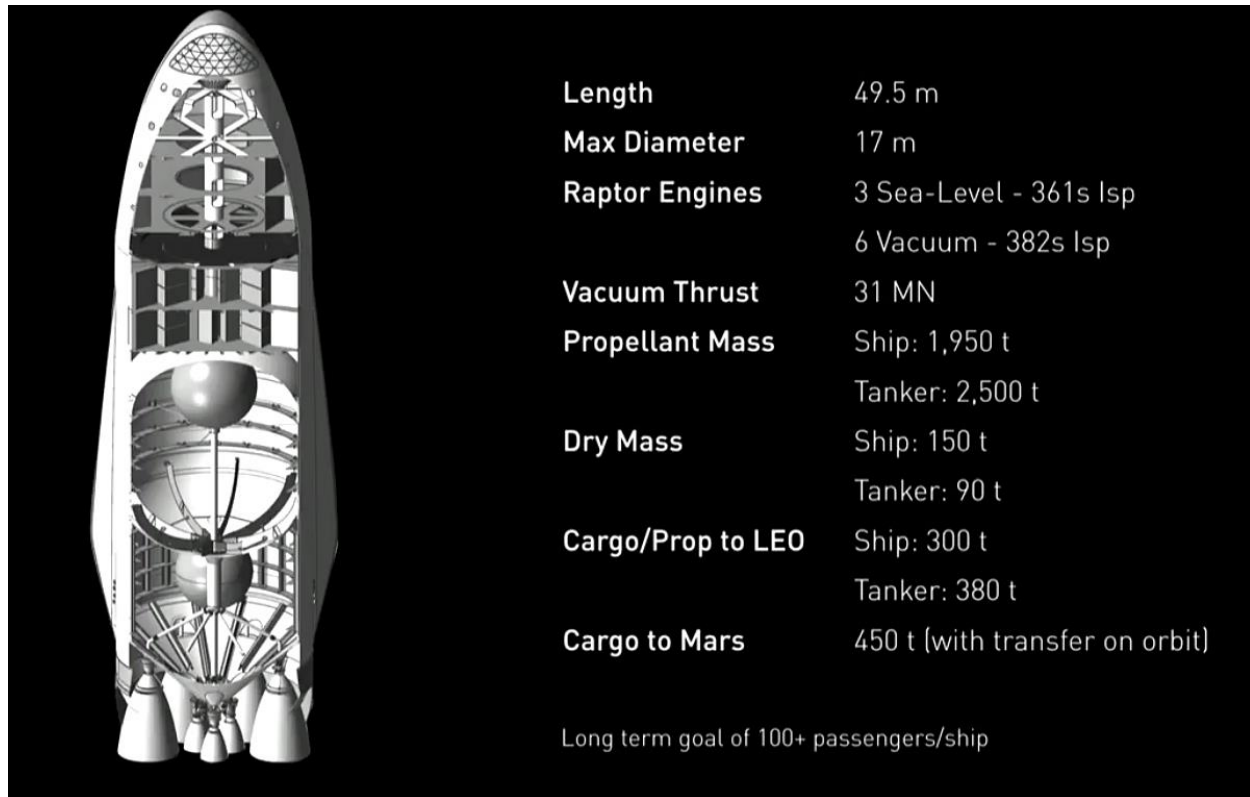
Figure 41. Mars Transport vehicle. Source: Space X.
