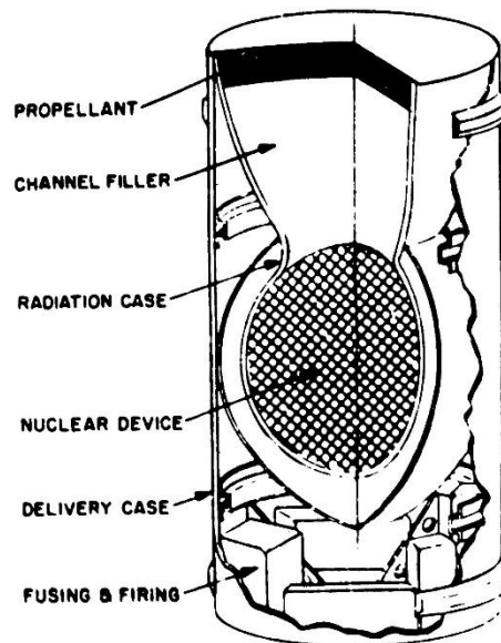
Figure 36. Design of a directed energy pulse unit with a heavy element propellant pusher plate. Propellant: Tungsten, Channel Filler: Beryllium oxide, Radiation case: Uranium.
