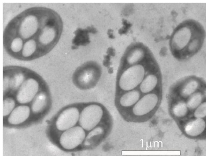
Figure 8. Transmission Electron Microscope (TEM) of cyanobacteria GFAJ-1. Source: Science, AAAS.
