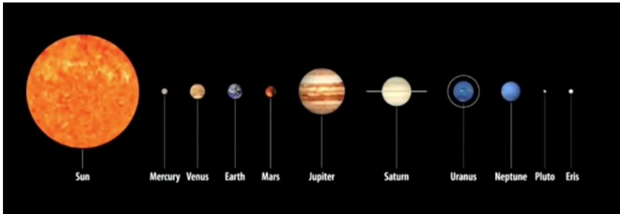
Figure 26. Comparison of solar system planets' sizes. Source: NASA.
