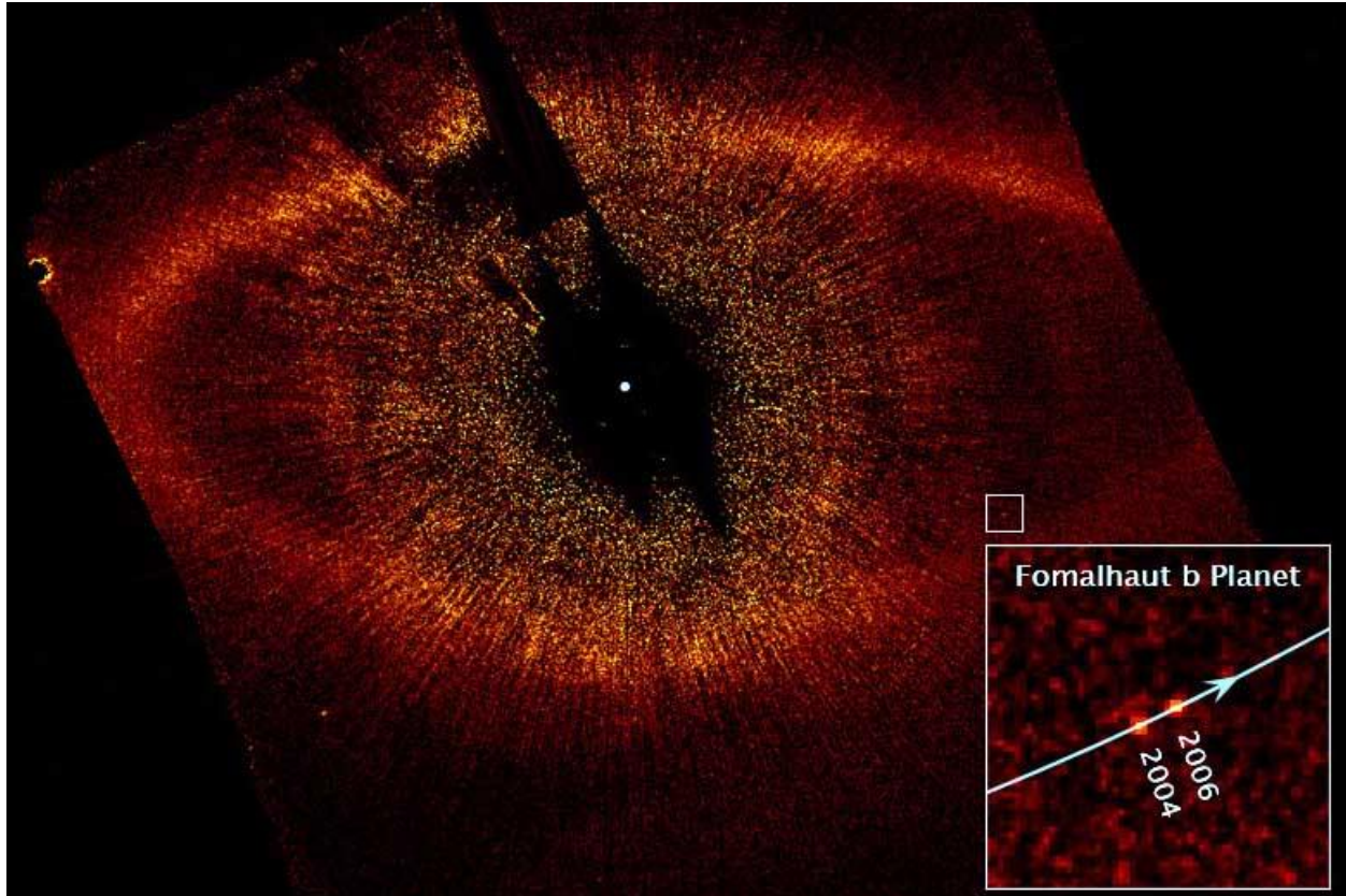
Figure 48. The Hubble Space Telescope was used to take the first visible-light snapshot of a planet orbiting another star. The images show the planet, named Fomalhaut b, as a tiny point source of light orbiting the nearby, bright southern star Fomalhaut, located 25 light-years away in the constellation Piscis Australis. A large debris disk about 21.5 billion miles across surrounds the star. Fomalhaut b is orbiting 1.8 billion miles inside the disk's sharp inner edge. Photo: NASA.
