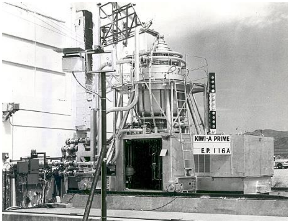
Figure 22. KIWI-A Prime nuclear rocket engine.
