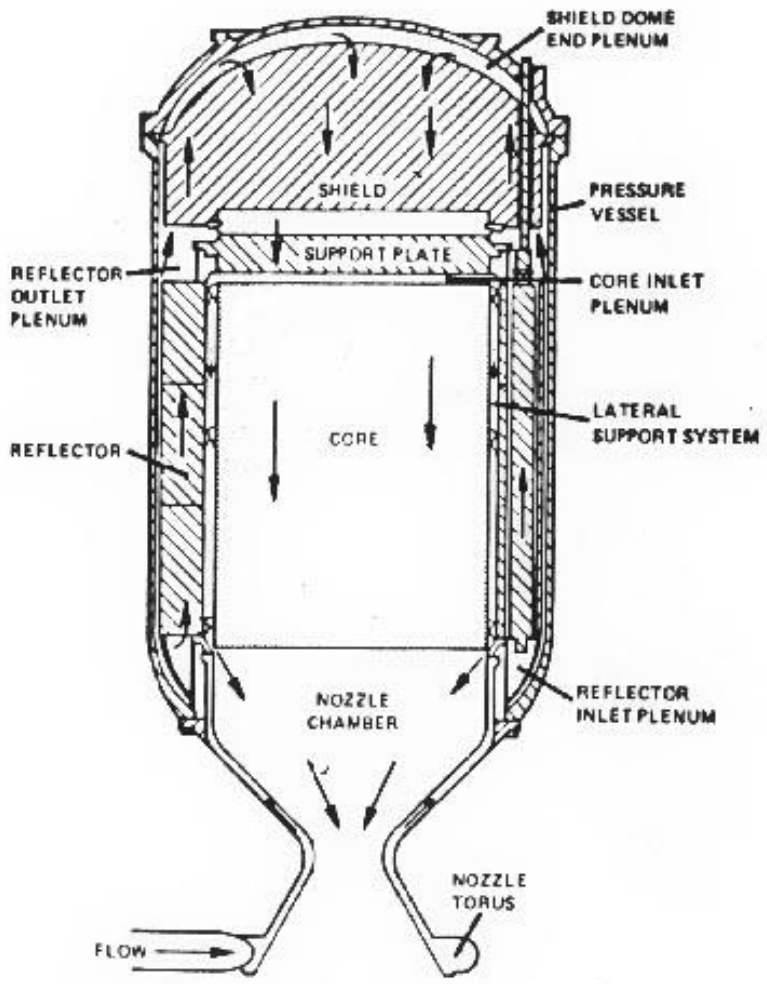
Figure 12. Reactor of solid core rocket.
