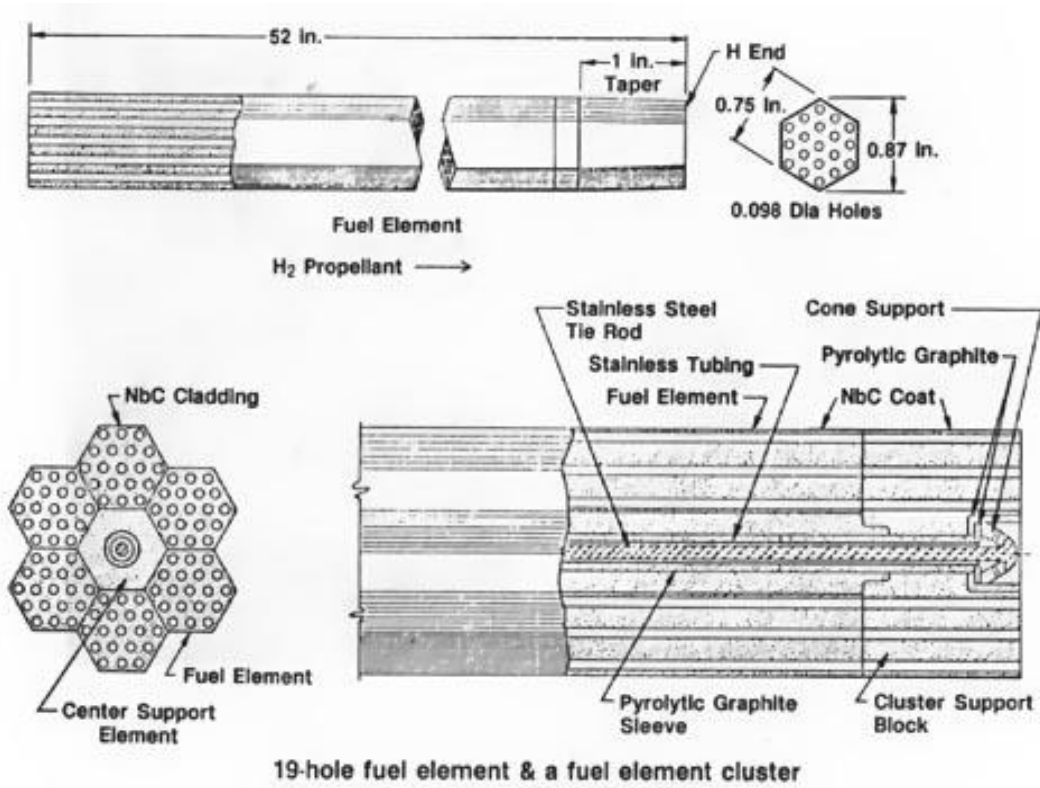
Figure 24. The KIWI B-4A Fuel Element Cluster.
